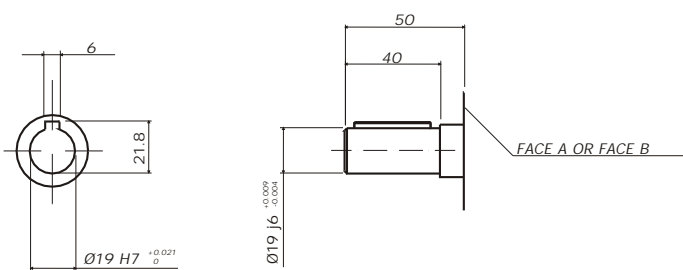
GEARBOX SHAFT DETAIL
